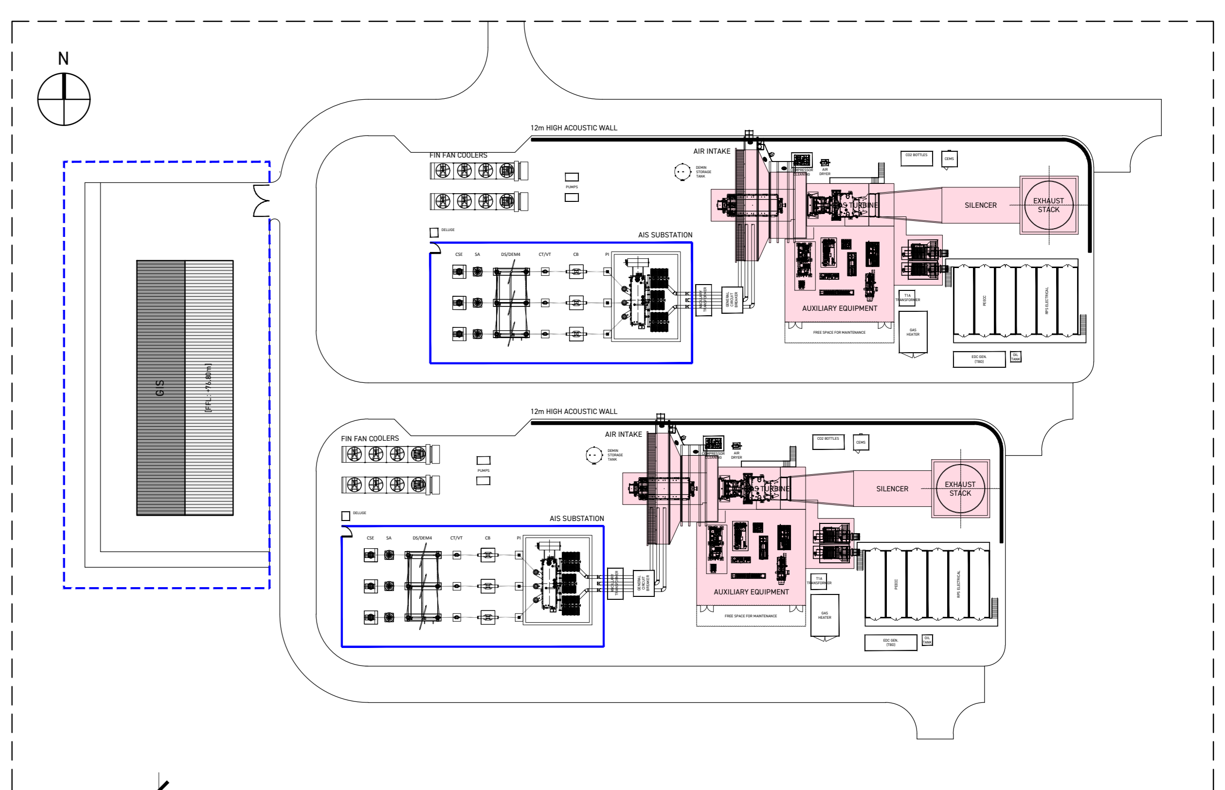
KEY PLAN
